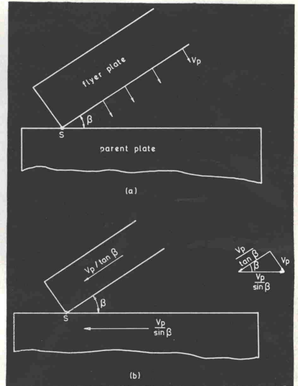
4 Change of co-ordinates for impacting plates. (a) Initial state; (b) change of co-ordinates.
